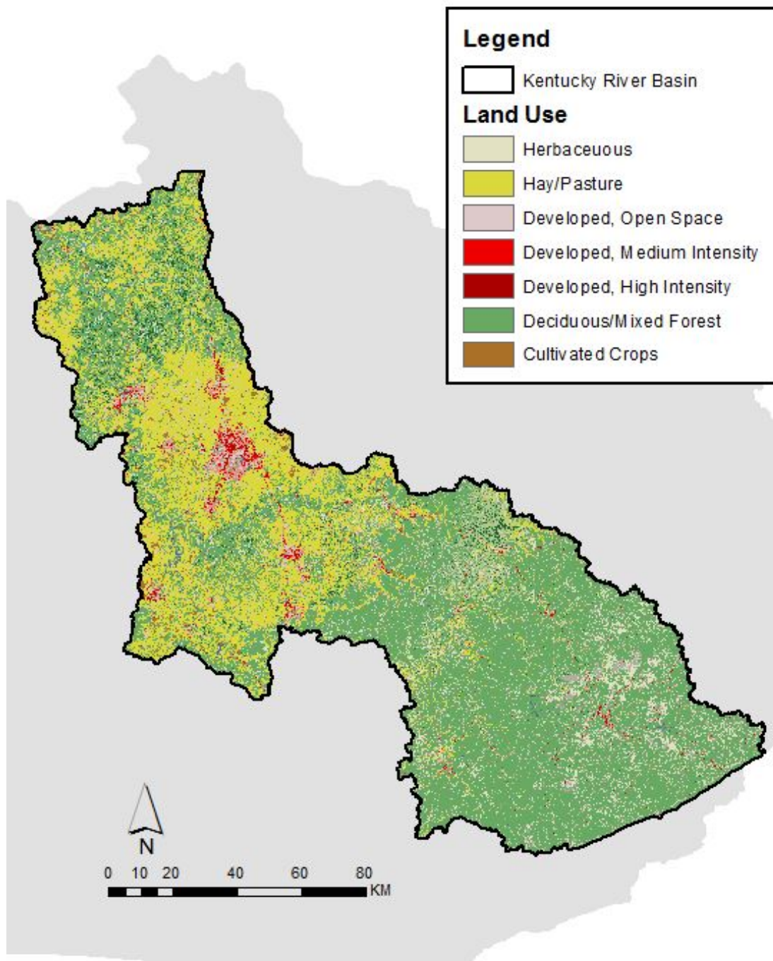
Figure 4.8: Kentucky River Basin land use
